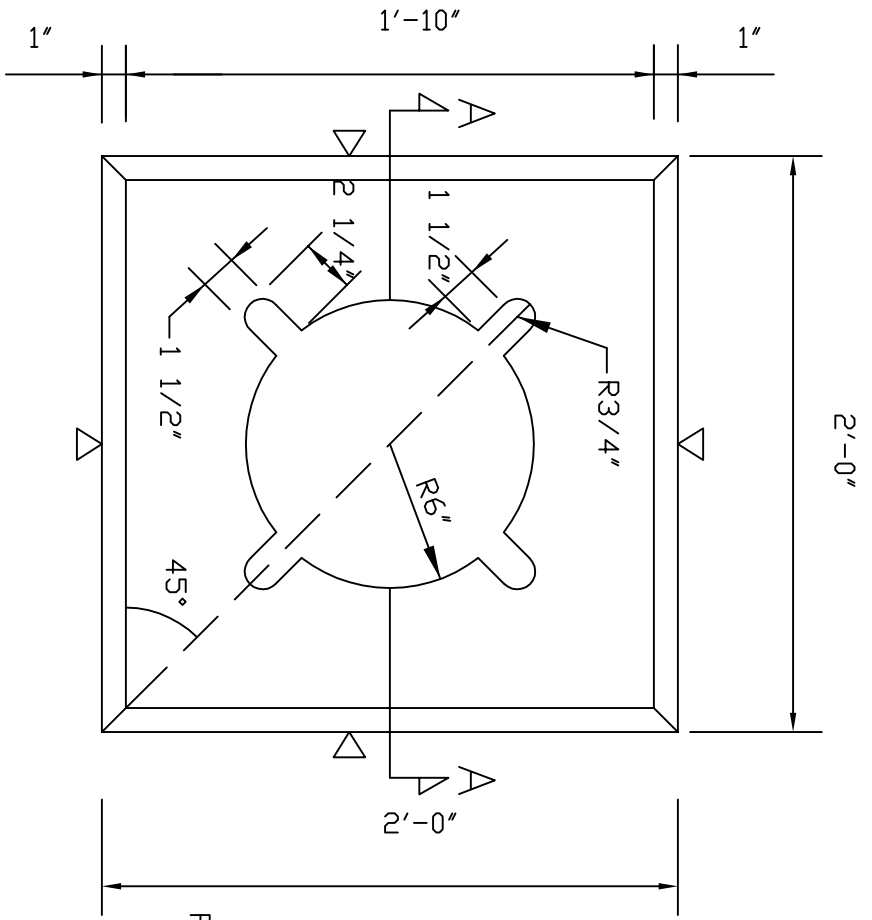
COLUMN BASE PLAN
